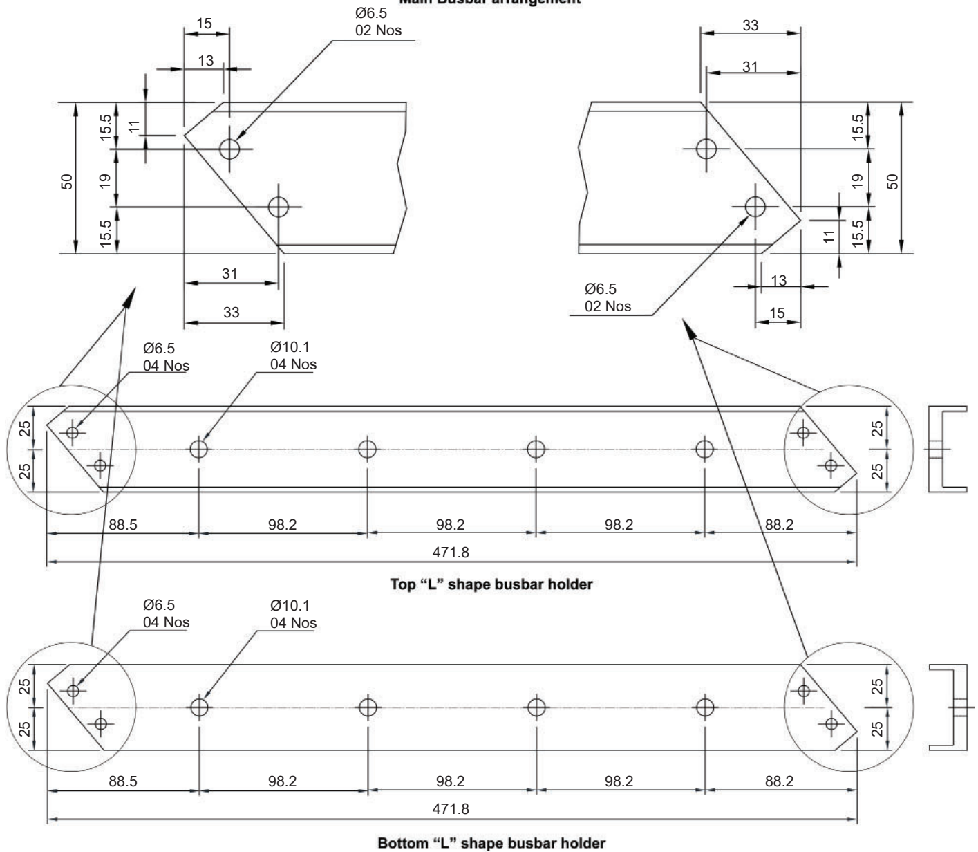
Main Busbar arrangement
